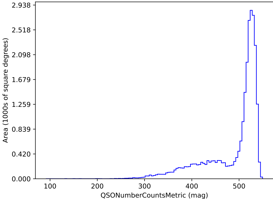
no_magell_roll_v3.4_10yrs r band and non-DD: QSONumberCountsMetric
