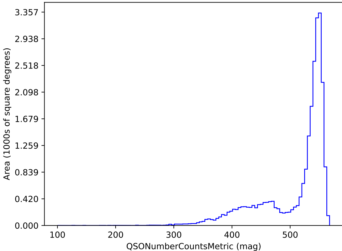
no_magell_roll_v3.4_10yrs i band and non-DD: QSONumberCountsMetric
