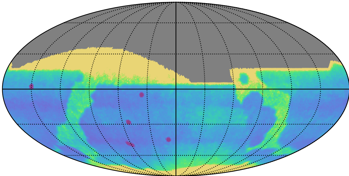
no_magell_roll_v3.4_10yrs : Proper Motion Uncert @ 24.0
