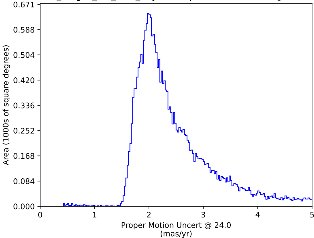
no_magell_roll_v3.4_10yrs : Proper Motion Uncert @ 24.0
