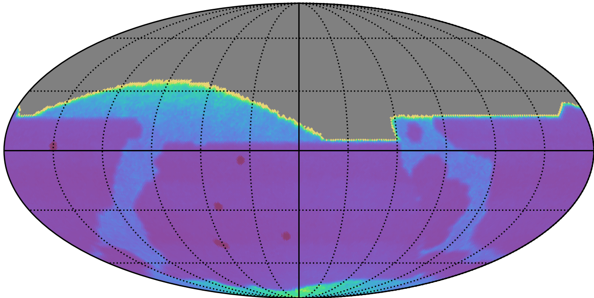
no_magell_roll_v3.4_10yrs : Proper Motion Uncert @ 20.5
