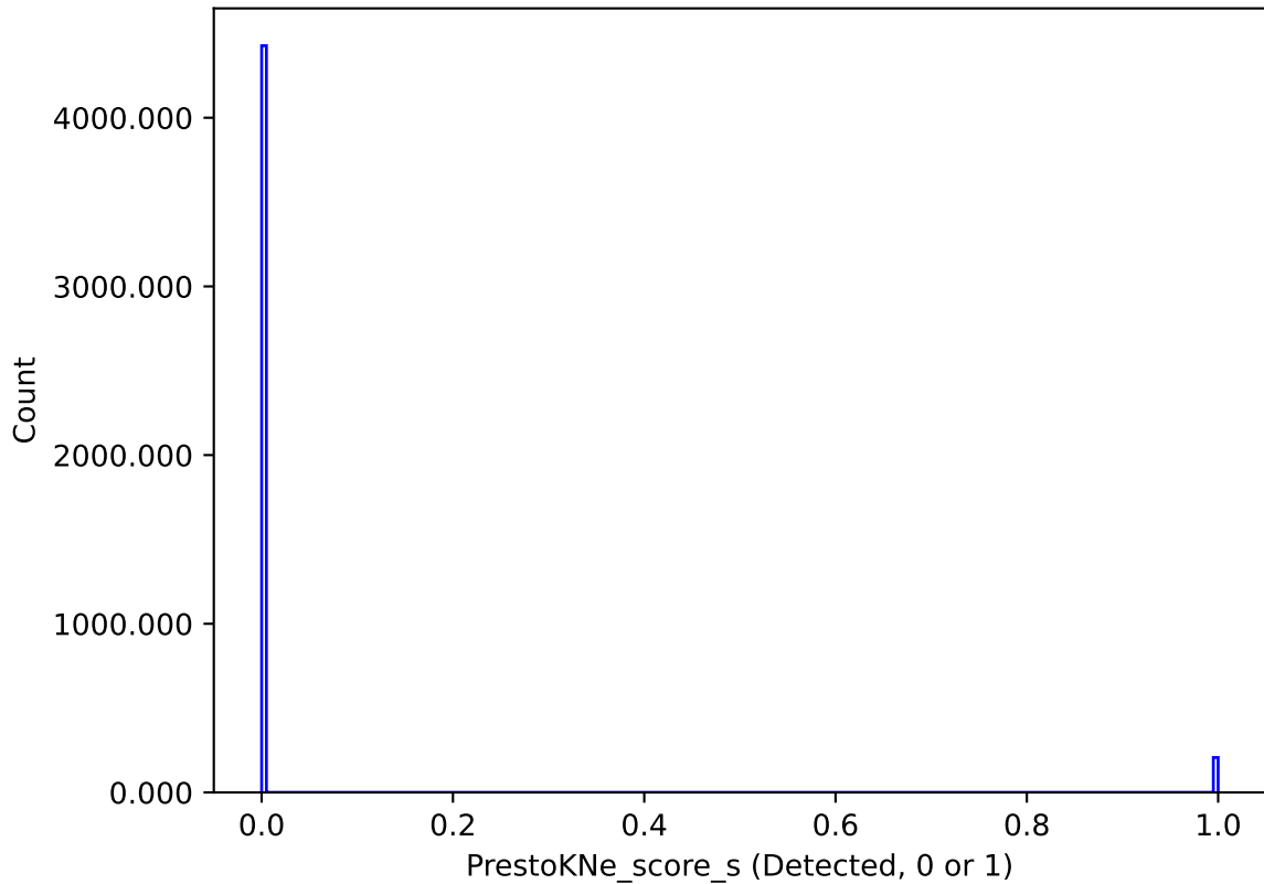
no_magell_roll_v3.4_10yrs : PrestoKNe_score_s
