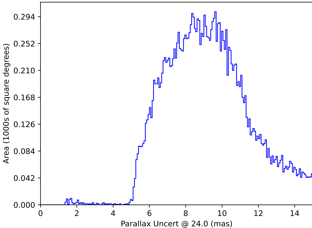
no_magell_roll_v3.4_10yrs : Parallax Uncert @ 24.0
