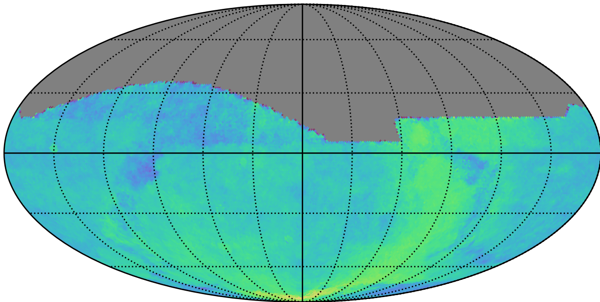
no_magell_roll_v3.4_10yrs : Parallax Coverage @ 24.0
