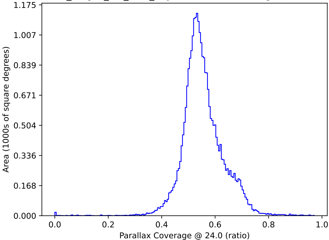
no_magell_roll_v3.4_10yrs : Parallax Coverage @ 24.0
