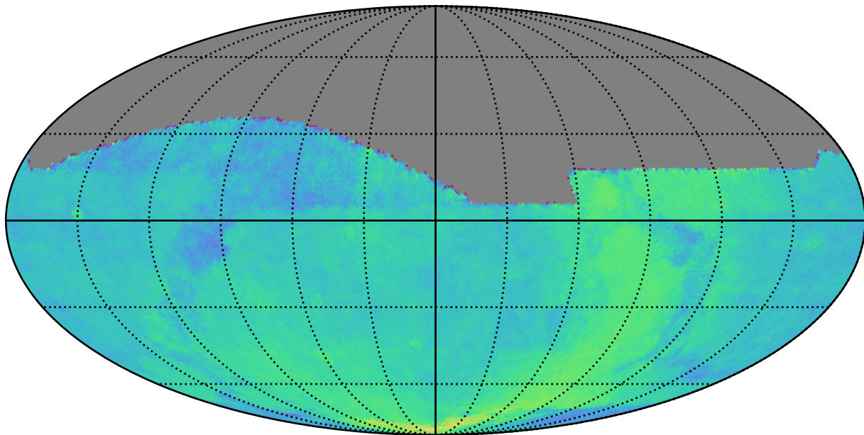
no_magell_roll_v3.4_10yrs : Parallax Coverage @ 22.4
