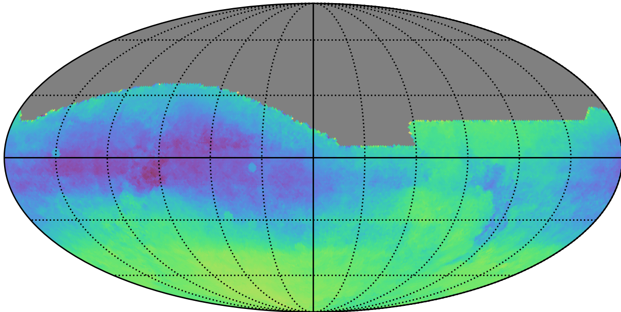
no_magell_roll_v3.4_10yrs : Parallax-DCR degeneracy @ 24.0
