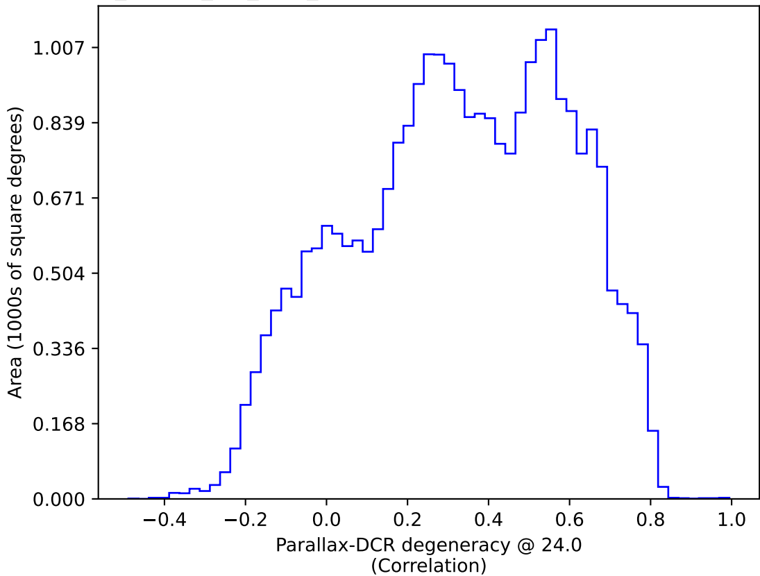
no_magell_roll_v3.4_10yrs : Parallax-DCR degeneracy @ 24.0
