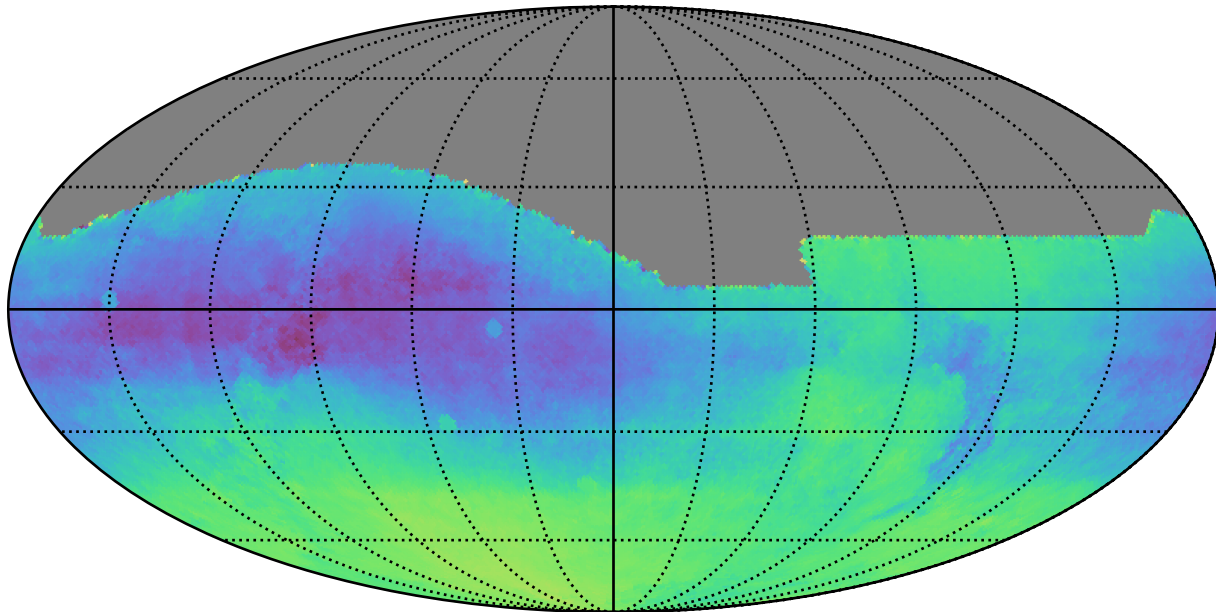
no_magell_roll_v3.4_10yrs : Parallax-DCR degeneracy @ 22.4
