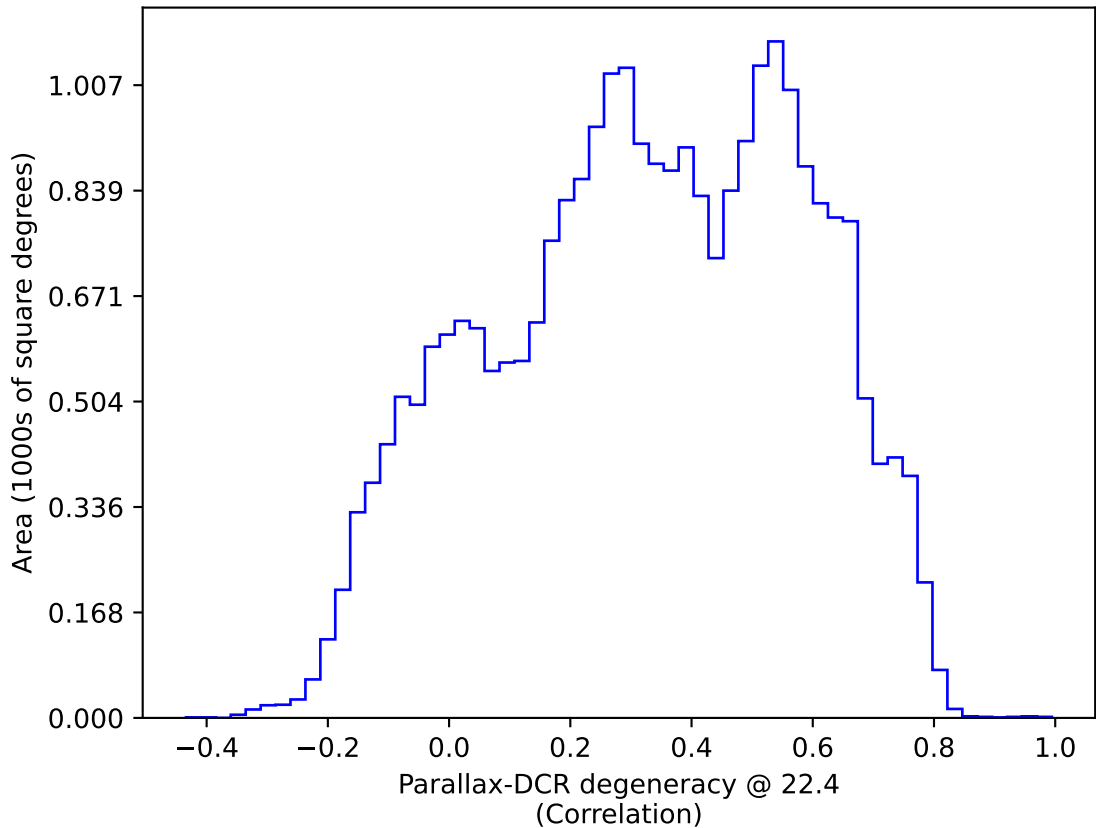
no_magell_roll_v3.4_10yrs : Parallax-DCR degeneracy @ 22.4
