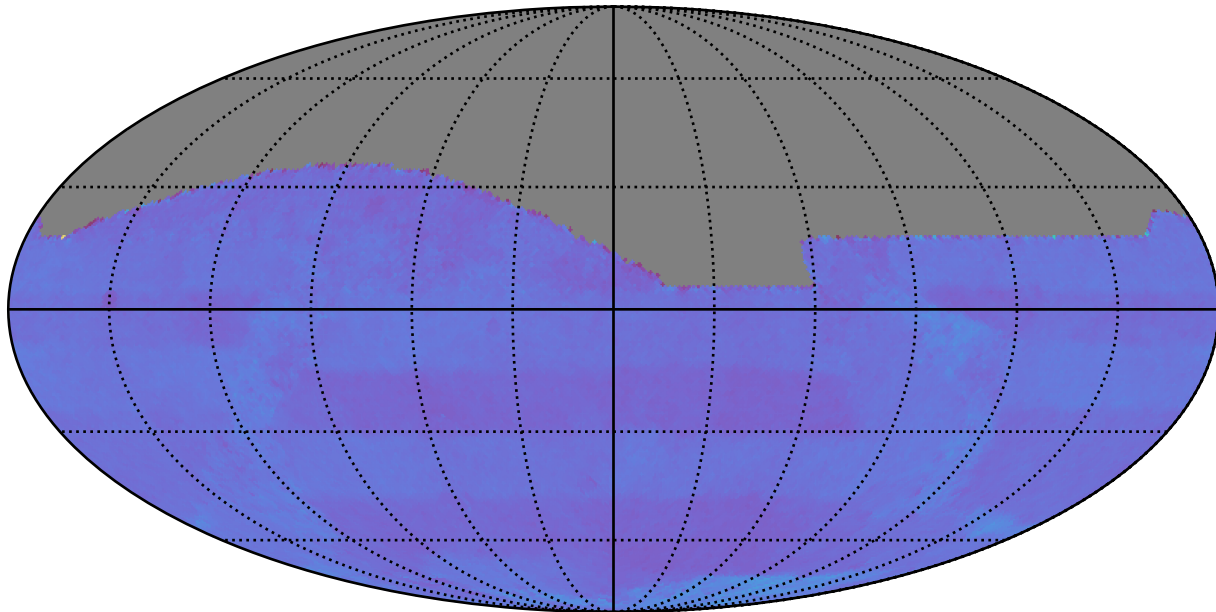
no_magell_roll_v3.4_10yrs : Normalized Proper Motion Uncert @ 24.0
