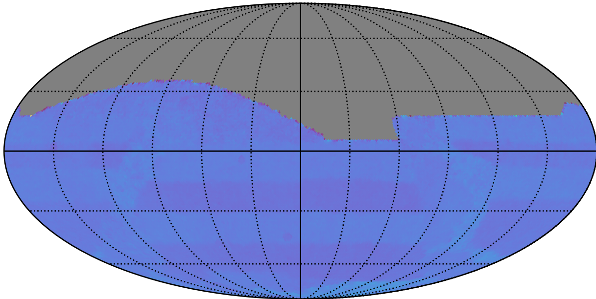
no_magell_roll_v3.4_10yrs : Normalized Proper Motion Uncert @ 20.5
