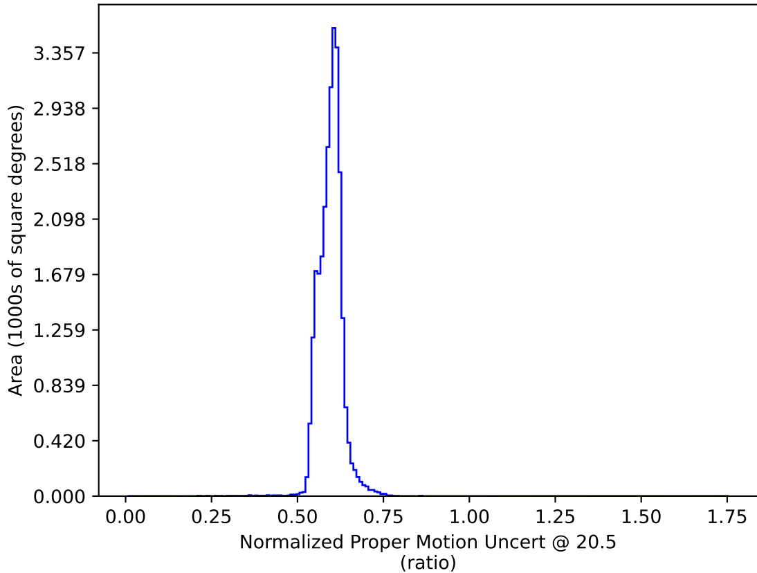
no_magell_roll_v3.4_10yrs : Normalized Proper Motion Uncert @ 20.5
