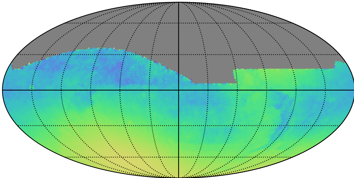
no_magell_roll_v3.4_10yrs : Normalized Parallax Uncert @ 24.0
