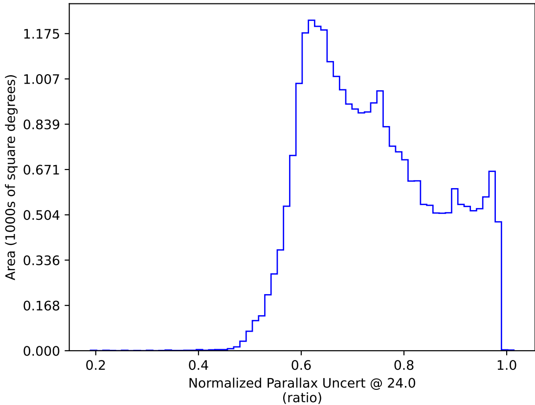
no_magell_roll_v3.4_10yrs : Normalized Parallax Uncert @ 24.0
