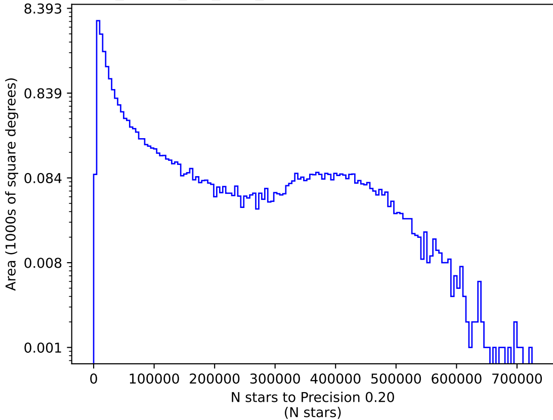
no_magell_roll_v3.4_10yrs z: N stars to Precision 0.20
