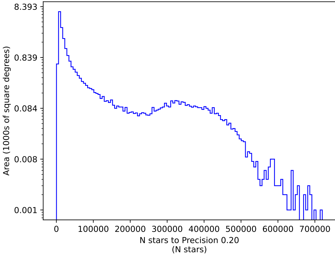
no_magell_roll_v3.4_10yrs y: N stars to Precision 0.20
