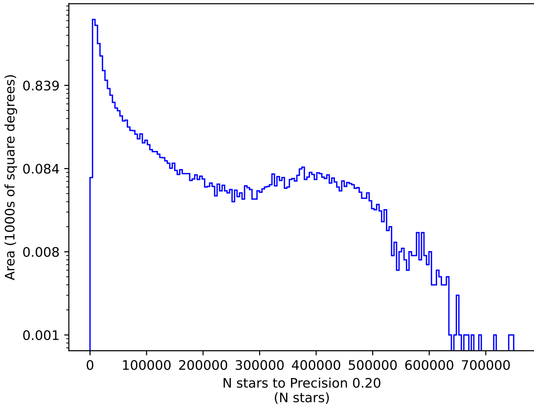
no_magell_roll_v3.4_10yrs r: N stars to Precision 0.20
