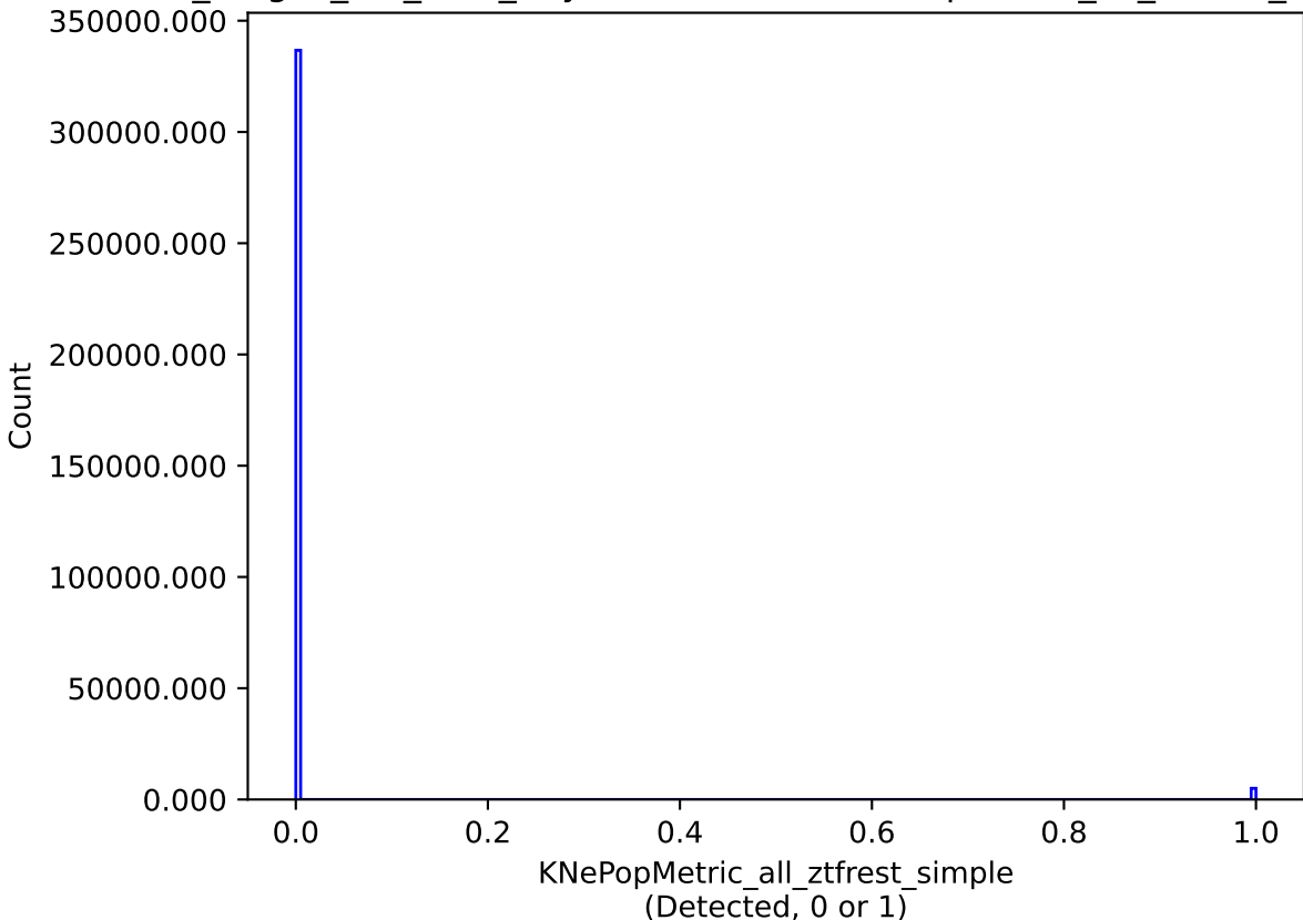
no_magell_roll_v3.4_10yrs all models: KNePopMetric_all_ztfrest_simple
