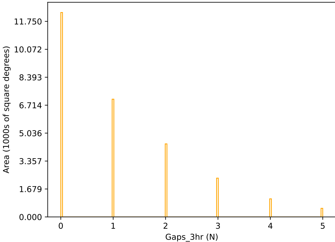
no_magell_roll_v3.4_10yrs r band: Gaps_3hr
