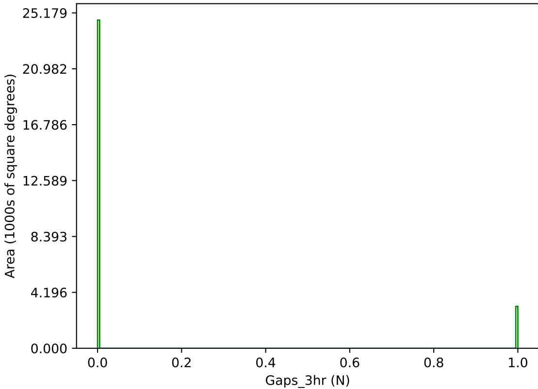
no_magell_roll_v3.4_10yrs g band: Gaps_3hr
