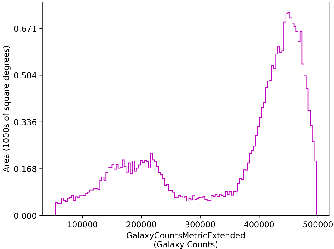
no_magell_roll_v3.4_10yrs z: GalaxyCountsMetricExtended
