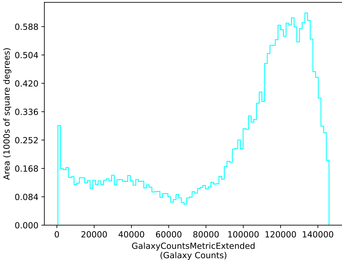
no_magell_roll_v3.4_10yrs u: GalaxyCountsMetricExtended
