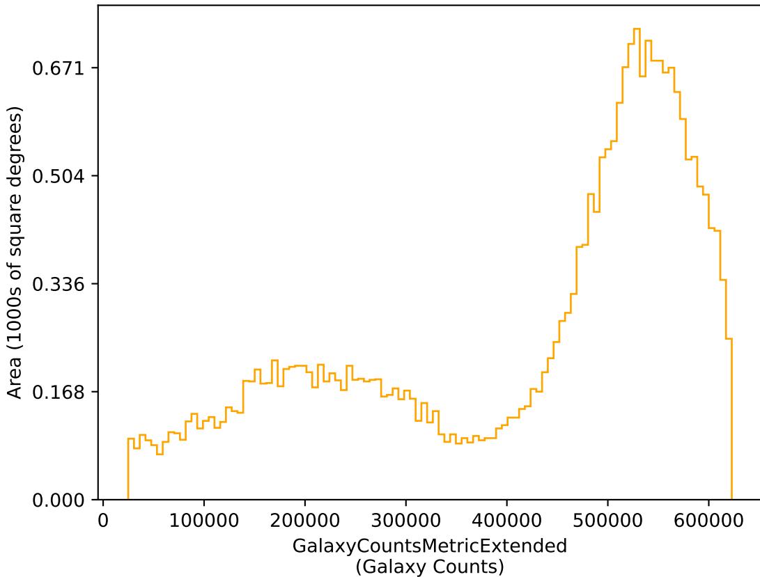
no_magell_roll_v3.4_10yrs r: GalaxyCountsMetricExtended
