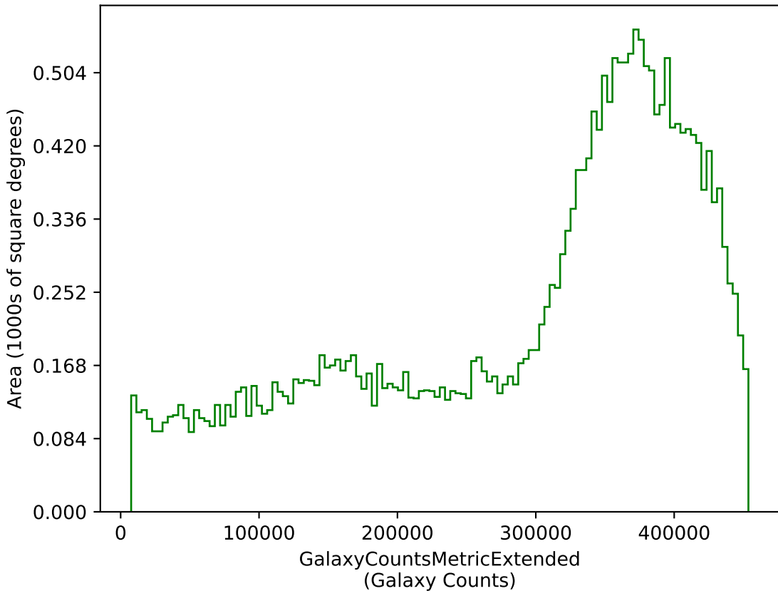
no_magell_roll_v3.4_10yrs g: GalaxyCountsMetricExtended
