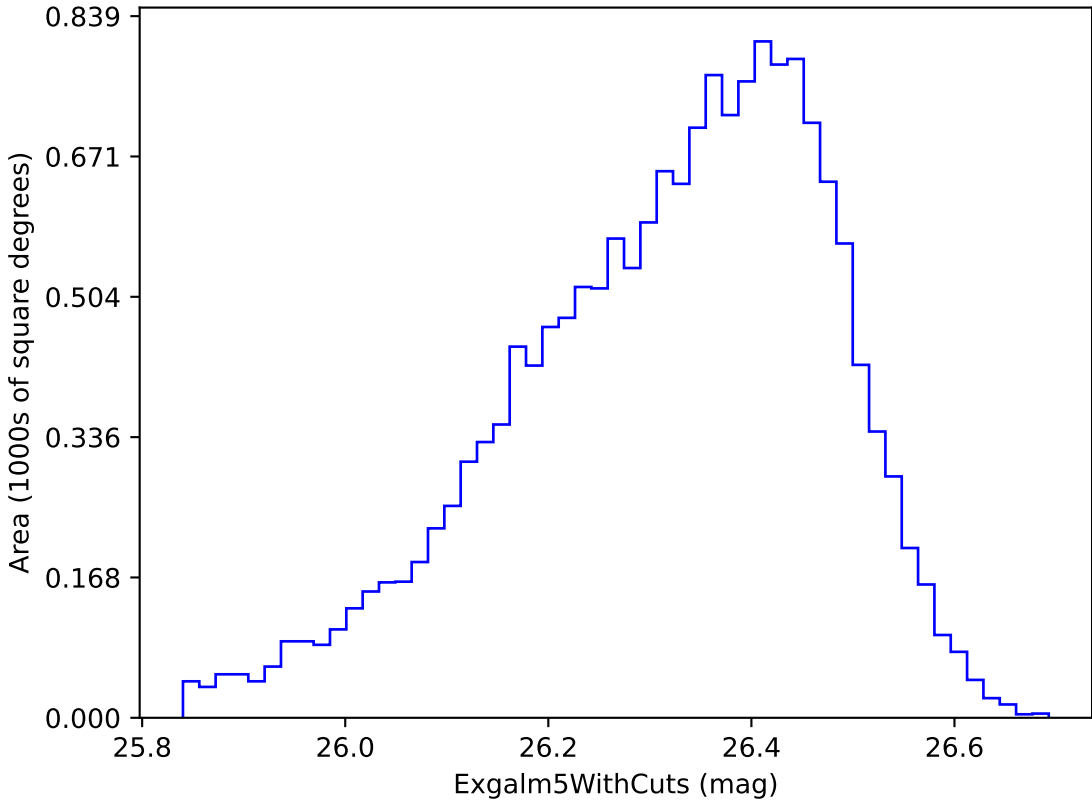
no_magell_roll_v3.4_10yrs i band non-DD year 9: ExgalM5WithCuts
