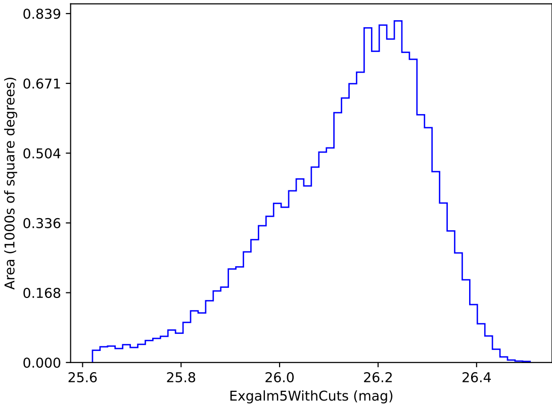
no_magell_roll_v3.4_10yrs i band non-DD year 6: ExgalM5WithCuts
