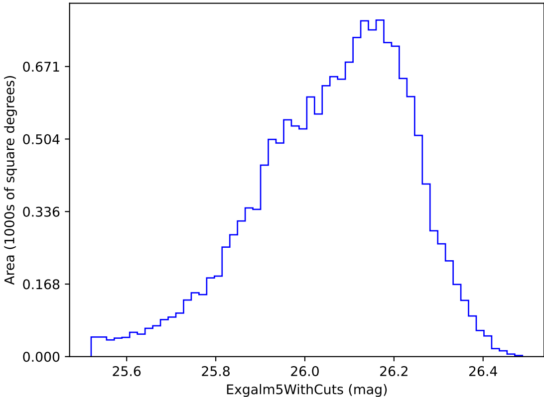
no_magell_roll_v3.4_10yrs i band non-DD year 5: Exgal5WithCuts
