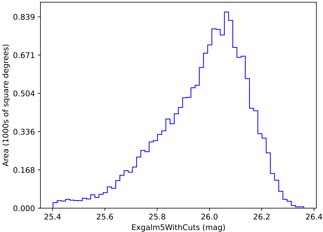
no_magell_roll_v3.4_10yrs i band non-DD year 4: ExgalM5WithCuts
