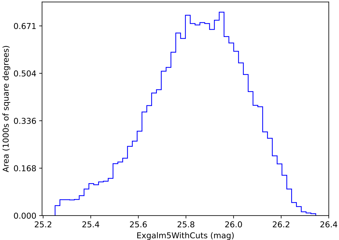
no_magell_roll_v3.4_10yrs i band non-DD year 3: ExgalM5WithCuts
