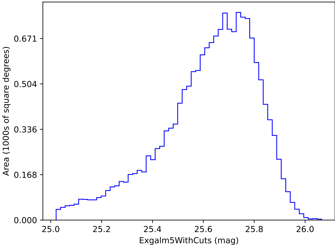
no_magell_roll_v3.4_10yrs i band non-DD year 2: ExgalM5WithCuts
