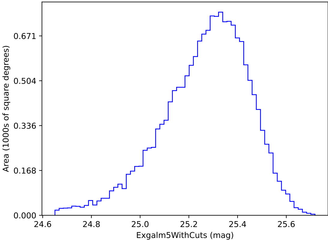
no_magell_roll_v3.4_10yrs i band non-DD year 1: ExgalM5WithCuts
