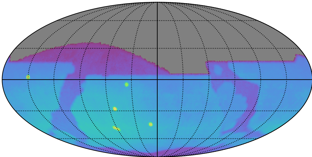
no_magell_roll_v3.4_10yrs : Brown Dwarf, L7
