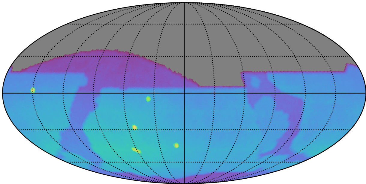
no_magell_roll_v3.4_10yrs : Brown Dwarf, L4
