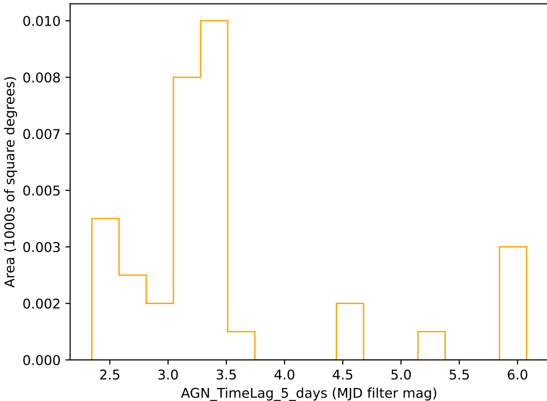
no_magell_roll_v3.4_10yrs r band: AGN_TimeLag_5_days
