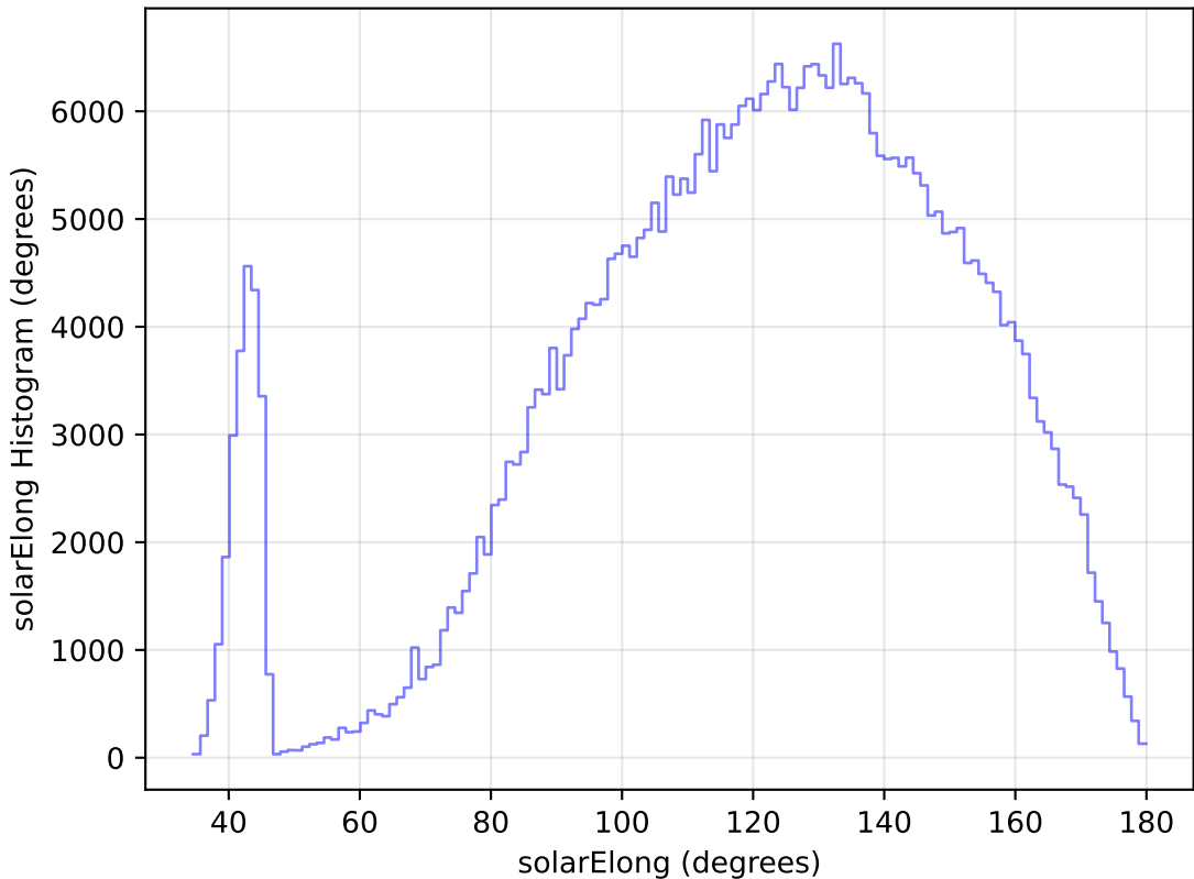
no_magell_roll_v3.4_10yrs WFD z band: solarElong Histogram
