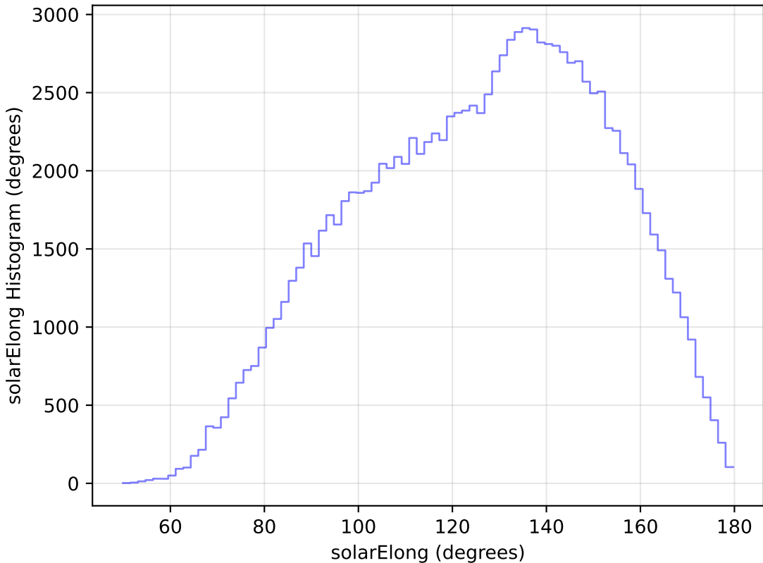
no_magell_roll_v3.4_10yrs WFD u band: solarElong Histogram
