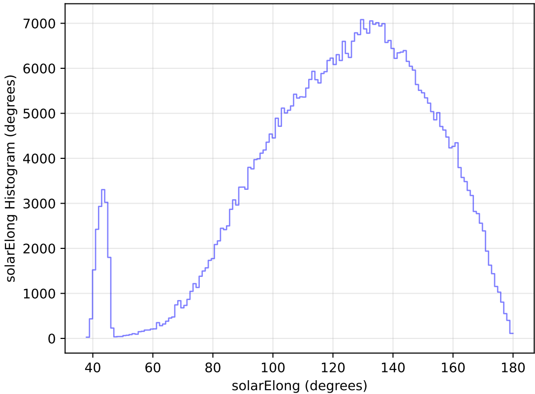
no_magell_roll_v3.4_10yrs WFD r band: solarElong Histogram
