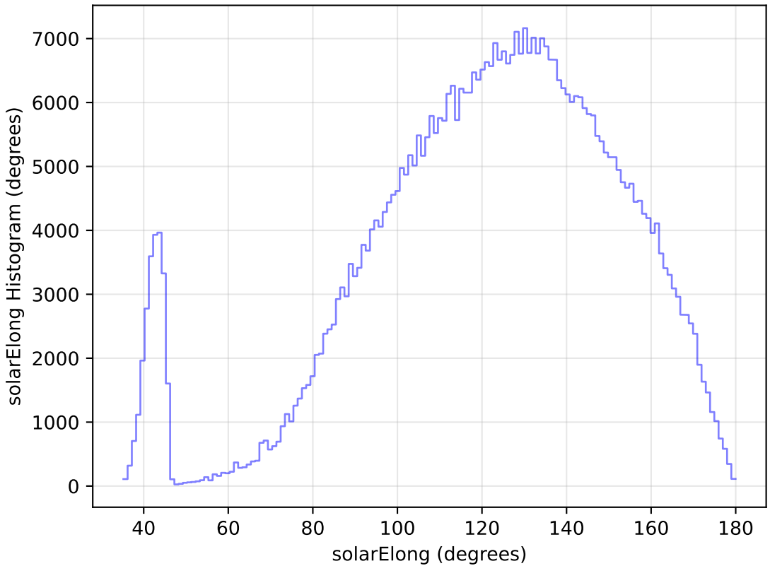
no_magell_roll_v3.4_10yrs WFD i band: solarElong Histogram
