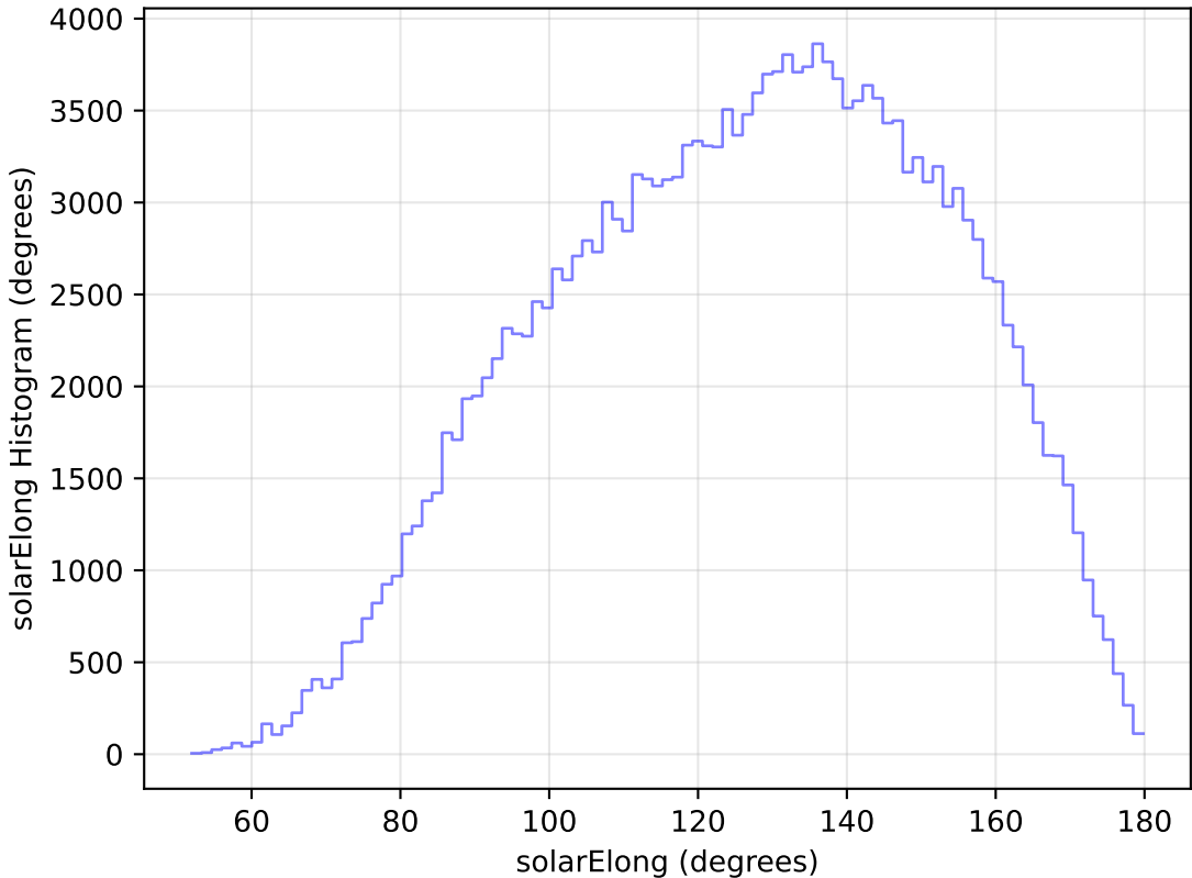
no_magell_roll_v3.4_10yrs WFD g band: solarElong Histogram
