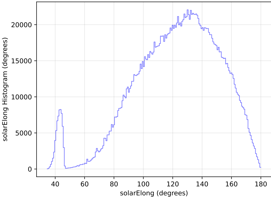
no_magell_roll_v3.4_10yrs WFD all bands: solarElong Histogram
