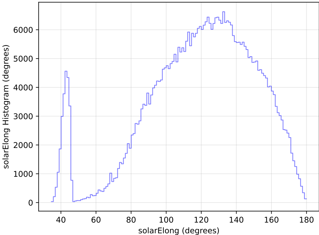
no_magell_roll_v3.4_10yrs All sky z band: solarElong Histogram
