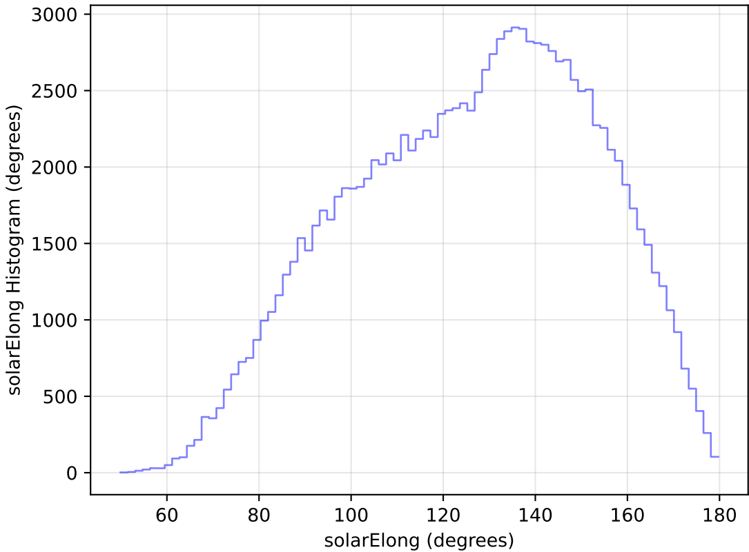
no_magell_roll_v3.4_10yrs All sky u band: solarElong Histogram
