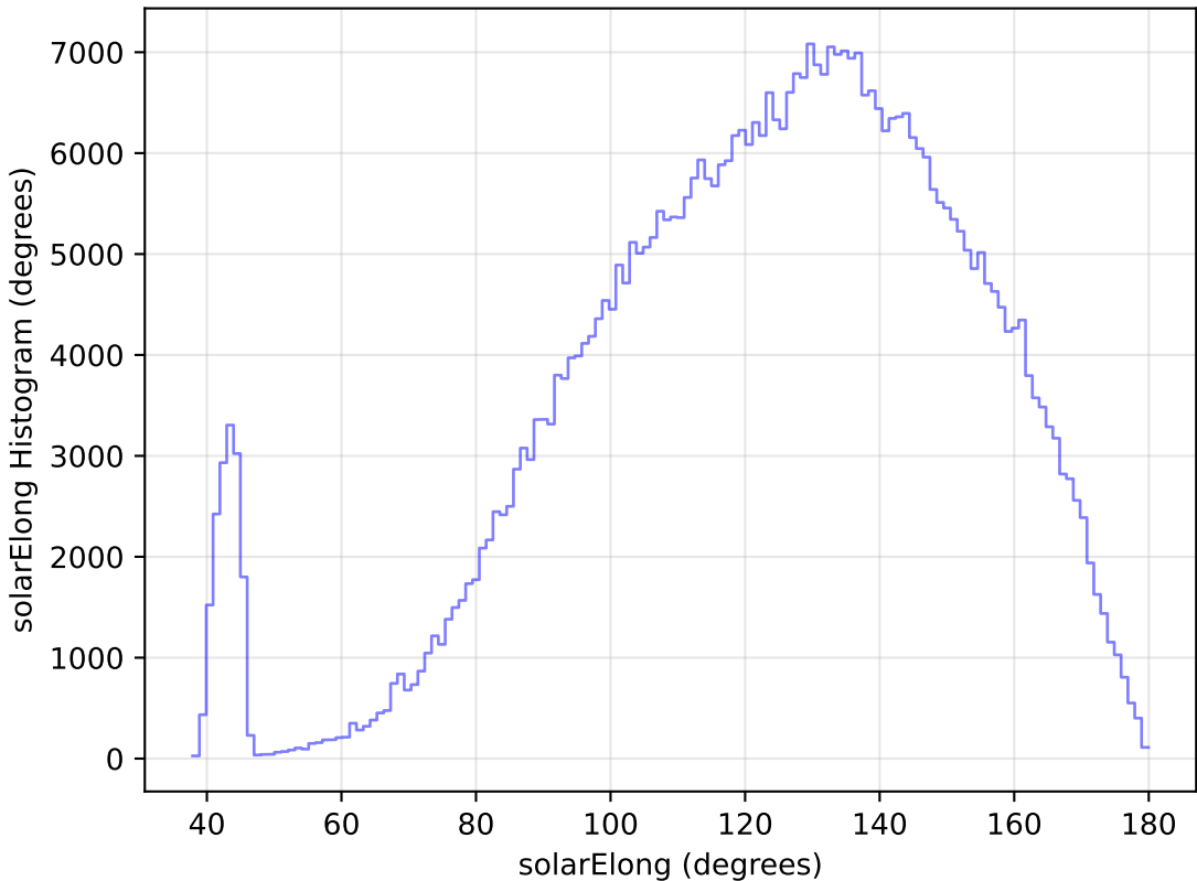
no_magell_roll_v3.4_10yrs All sky r band: solarElong Histogram
