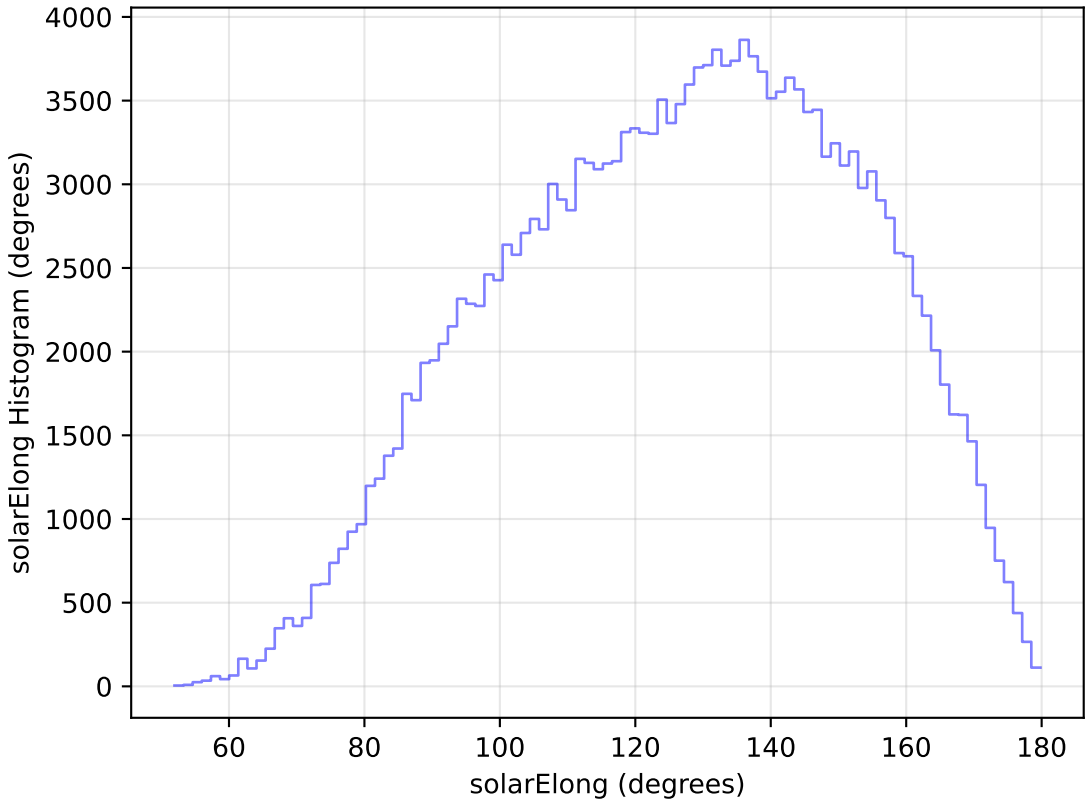
no_magell_roll_v3.4_10yrs All sky g band: solarElong Histogram
