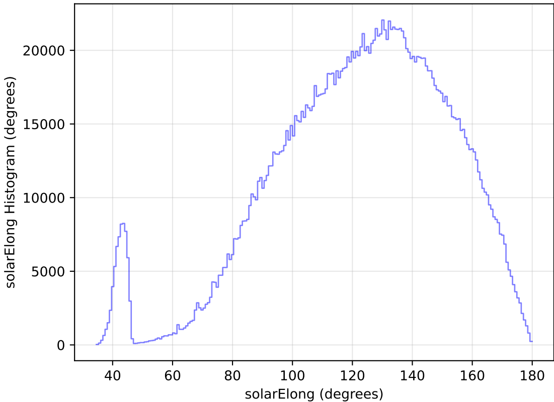
no_magell_roll_v3.4_10yrs All sky all bands: solarElong Histogram
